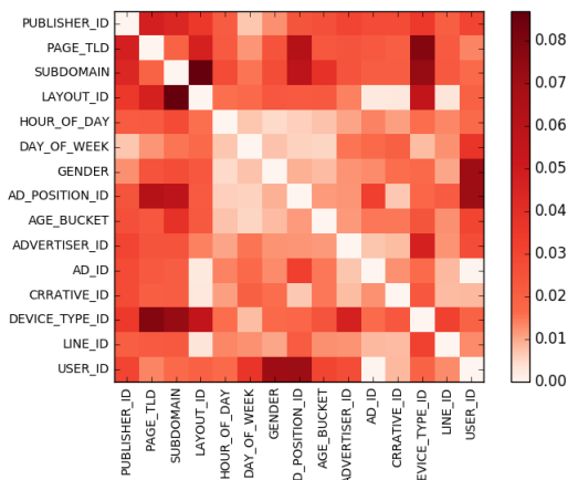
(c) Heat map of learned field interaction strengths of FwFMs. Pearson correlation coefficient with mutual informations: 0.1544.
